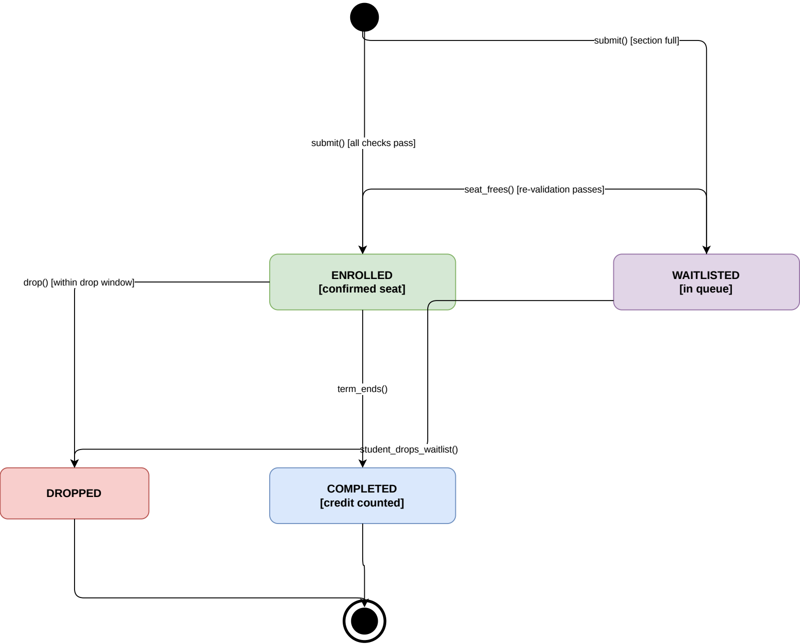
State Machine Diagram — Enrollment Lifecycle
