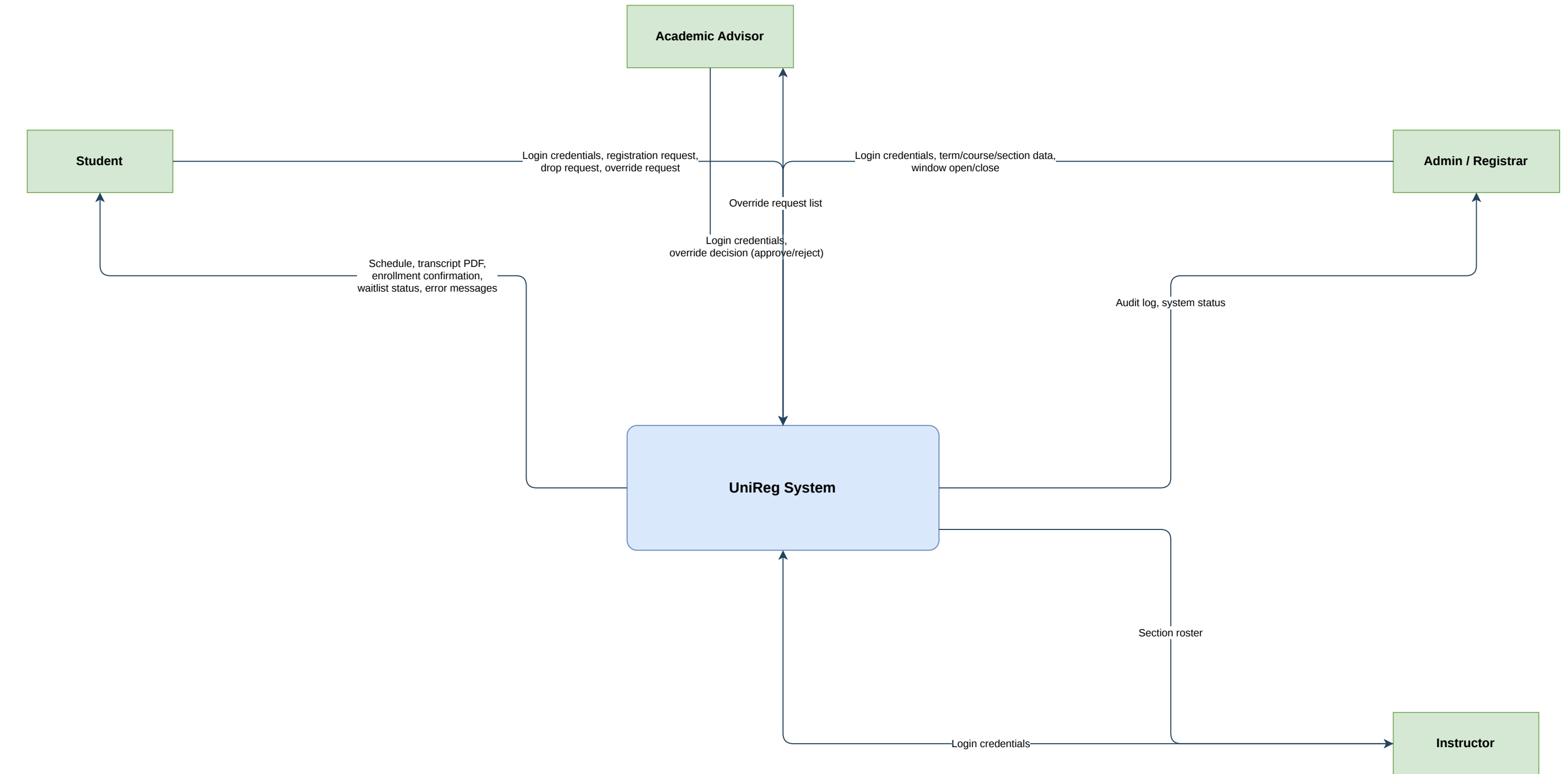
Context Diagram — UniReg System (DFD Level 0)
