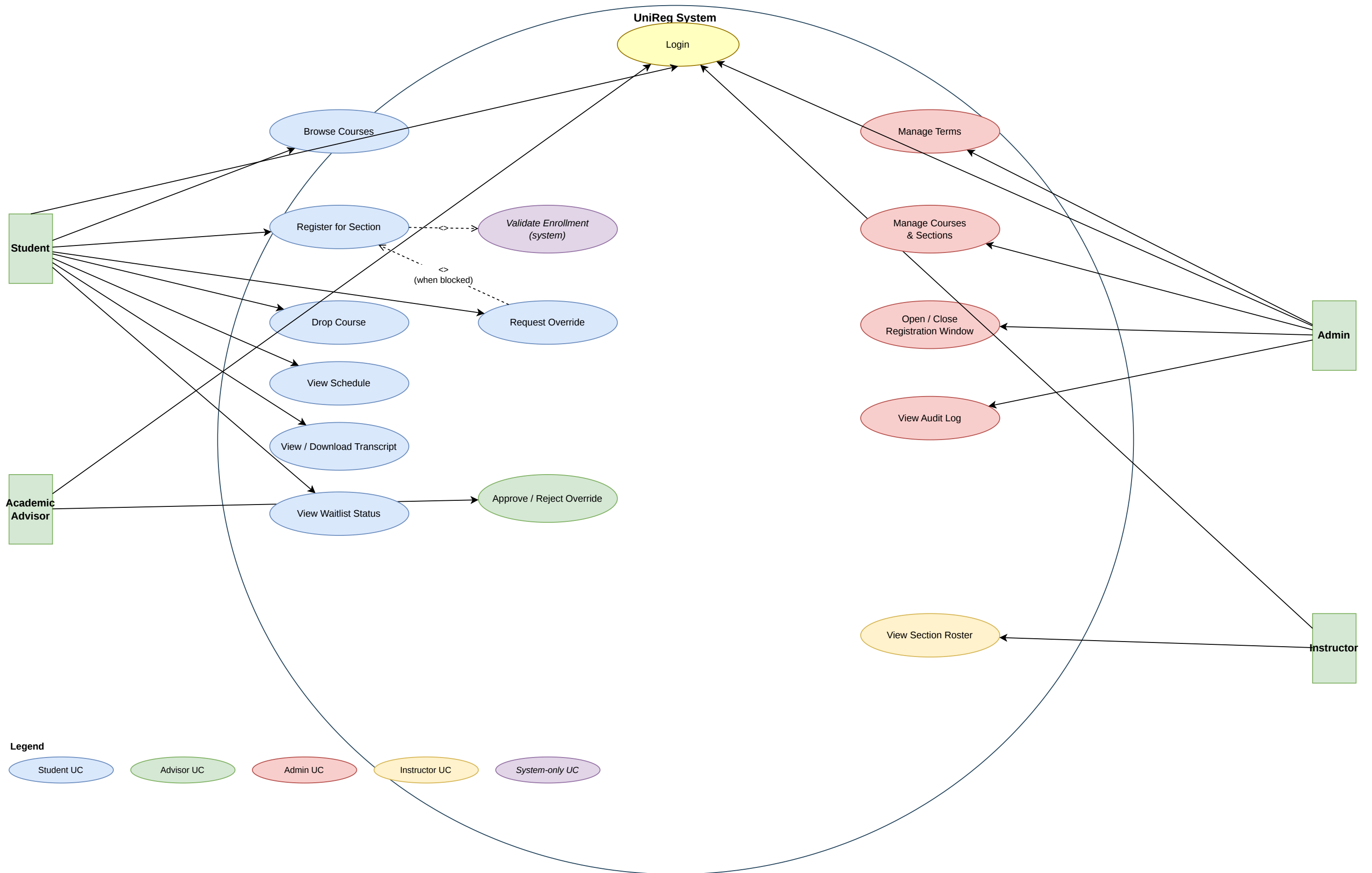
Use Case Diagram — UniReg System
